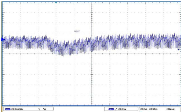
FIGURE 18. LOAD TRANSIENT (0A TO 50A STEP, SLEW_RATE = 2.5A/ \mu s)
