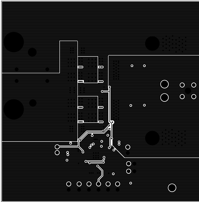
FIGURE 7. 4 th LAYER
