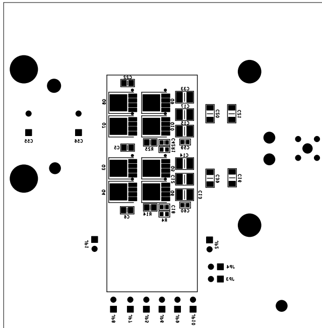
FIGURE 11. BOTTOM SILKSCREEN
