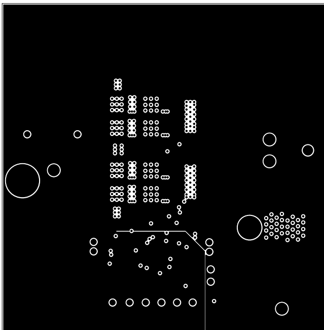
FIGURE 5. 2 nd LAYER
