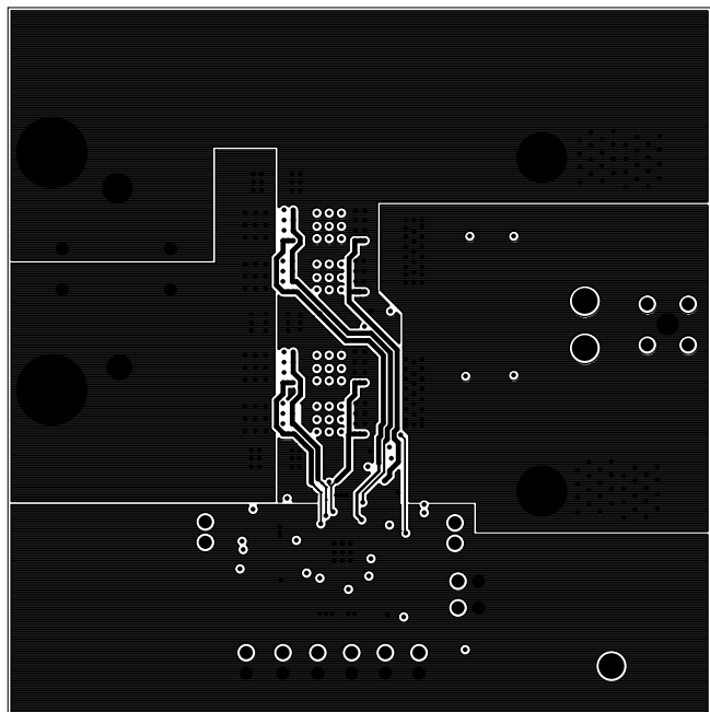
FIGURE 6. 3 rd LAYER
