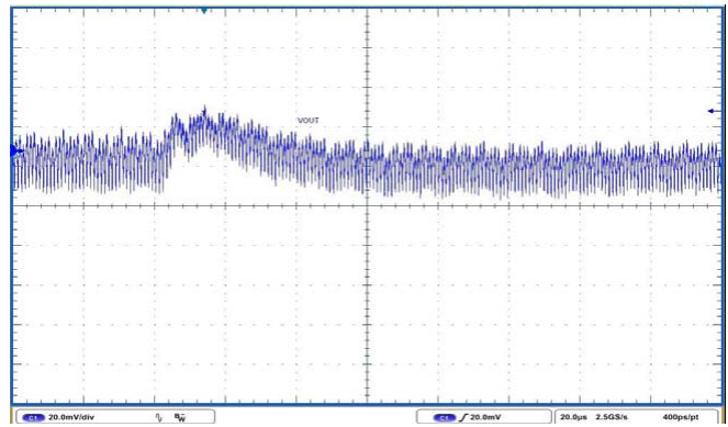
FIGURE 19. LOAD TRANSIENT (50A TO 0A STEP, SLEW_RATE = 2.5A/ \mu s)
