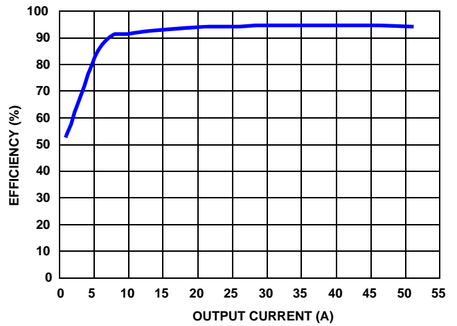
FIGURE 13. EFFICIENCY (12V V_{IN} AND 3.3V V_{OUT} )
