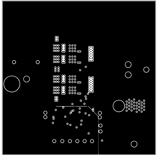
FIGURE 8. 5 th LAYER
